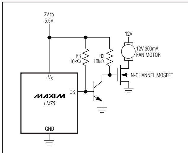
Figure 8. Fan Control
