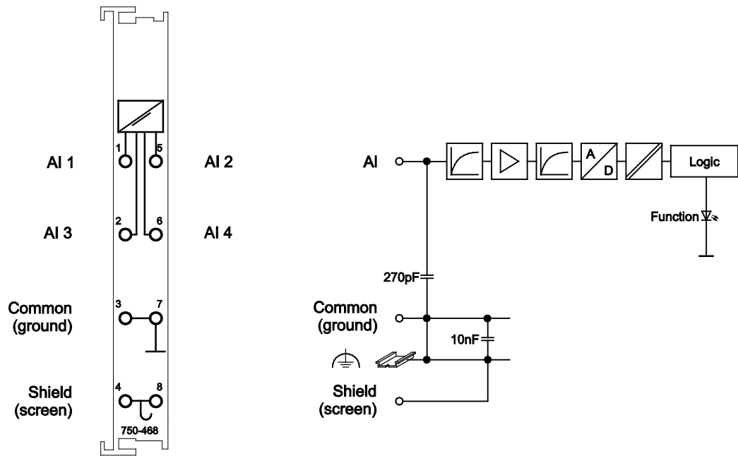
Figure 5: Schematic Diagram
