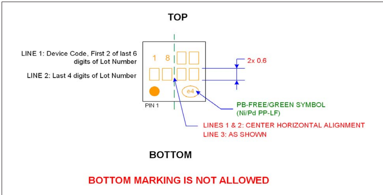
FIGURE 7-3: CAP1106 Package Markings
