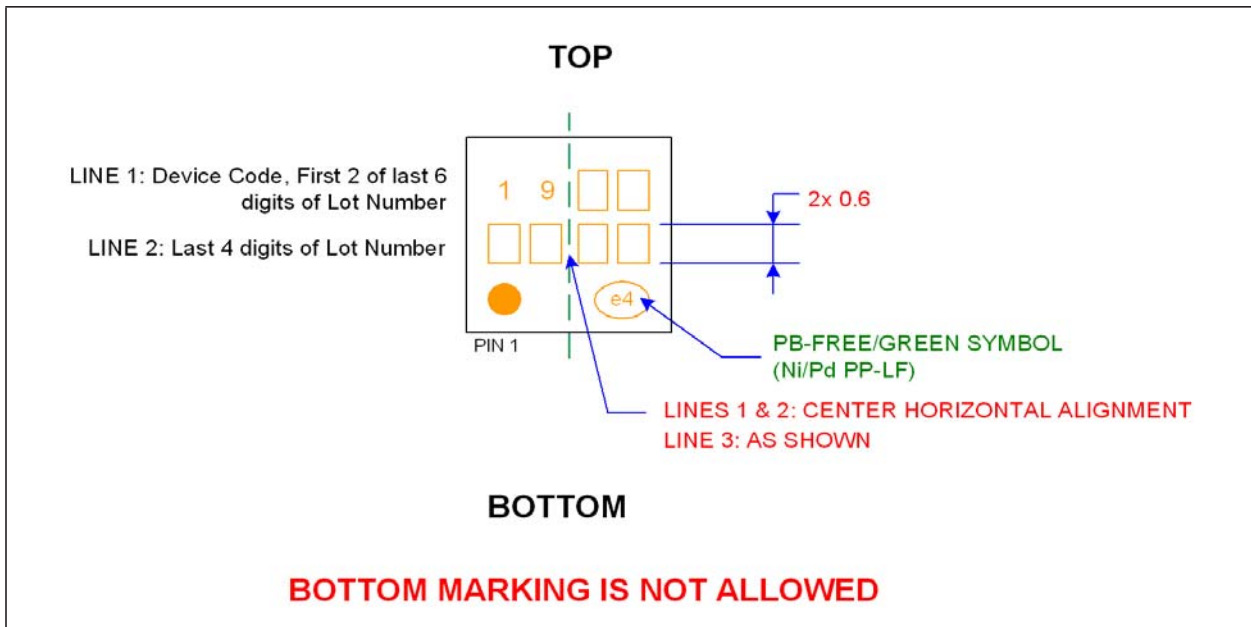
FIGURE 7-4: CAP1106 with BC-Link Support Package Markings
