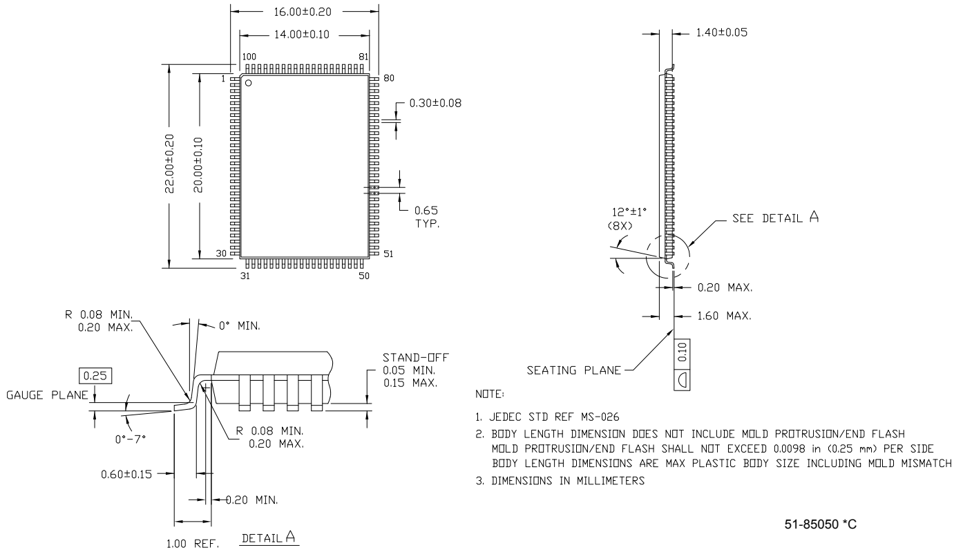
Figure 11. 100-pin Thin Plastic Quad Flatpack (14 × 20 × 1.4 mm) A101
