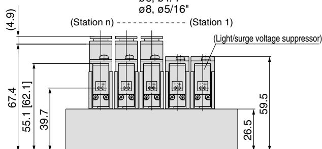
L plug connector (L)
