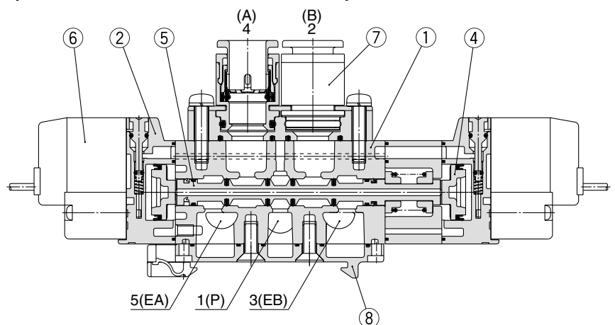
3 position closed center / exhaust center / pressure center
