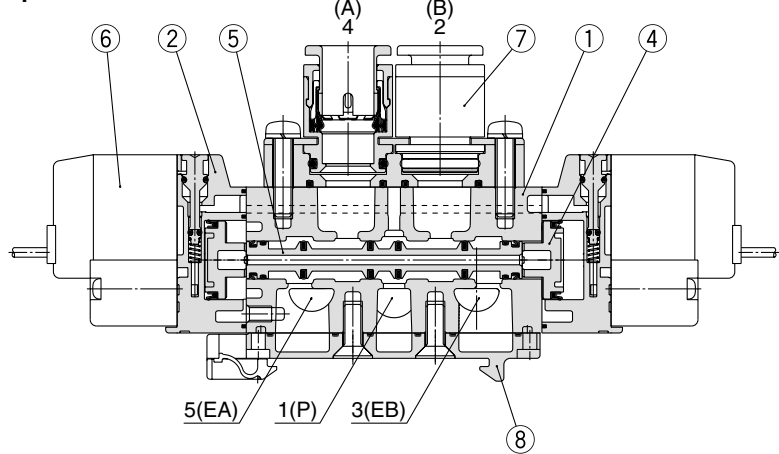
3 position closed center / exhaust center / pressure center
