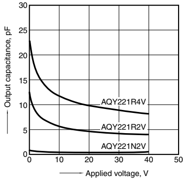
13. Output capacitance vs. applied voltage characteristics Measured portion: between terminals 3 and 4 Frequency: 1 MHz, 30m Vrms Ambient temperature: 25°C 77°F
