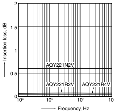
15. Insertion loss vs. frequency characteristics (50Ω impedance) Measured portion: between terminals 3 and 4 Ambient temperature: 25°C 77°F
