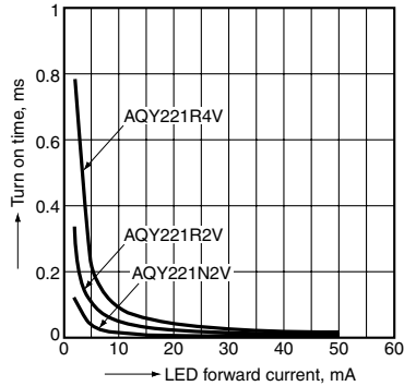
11. Turn on time vs. LED forward current characteristics Measured portion: between terminals 3 and 4 Load voltage: 10V (DC) Continuous load current: AQY221R4V 500mA (DC), AQY221R2V 250mA (DC), AQY221N2V 80mA (DC) Ambient temperature: 25°C 77°F
