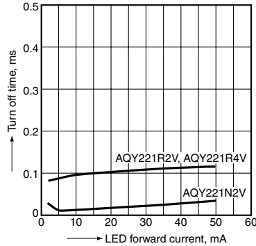
12. Turn off time vs. LED forward current characteristics Measured portion: between terminals 3 and 4 Load voltage: 10V (DC) Continuous load current: AQY221R4V 500mA (DC), AQY221R2V 250mA (DC), AQY221N2V 80mA (DC) Ambient temperature: 25°C 77°F
