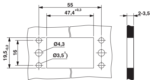
Housing cutout
