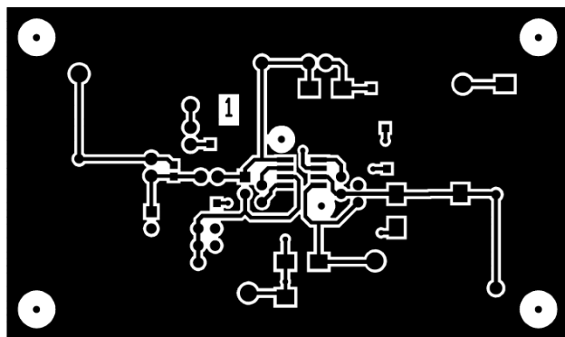
Figure 35. AD737 Evaluation Board—Component-Side Copper
