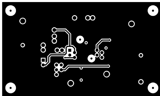
Figure 36. AD737 Evaluation Board—Secondary-Side Copper
