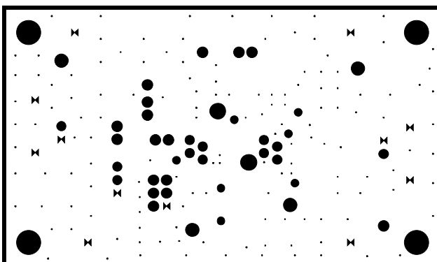
Figure 38. AD737 Evaluation Board—Internal Ground Plane
