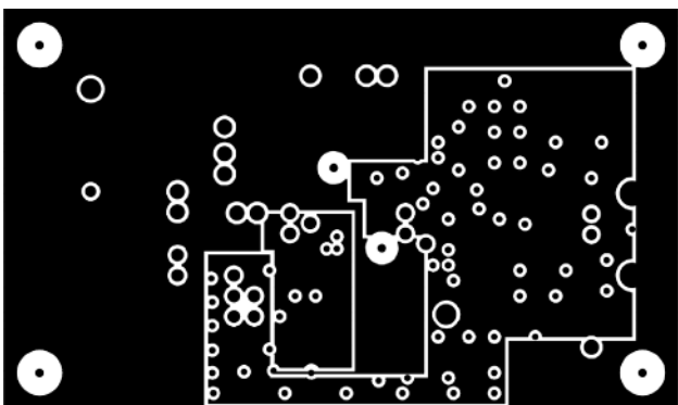
Figure 37. AD737 Evaluation Board—Internal Power Plane
