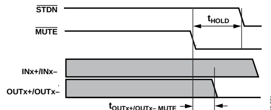
Figure 3. Timing Diagram Mute
