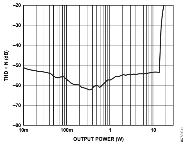
Figure 12. THD + N vs. Output Power, 15 V, 6 \Omega
