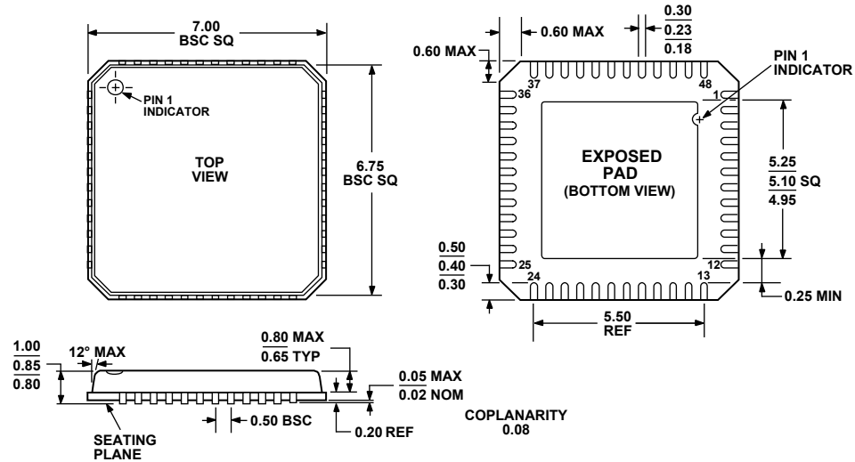
Figure 32. 48-Lead Lead Frame Chip Scale Package [LFCSP_VQ] 7 mm x 7 mm Body, Very Thin Quad (CP-48-1) Dimensions shown in millimeters
