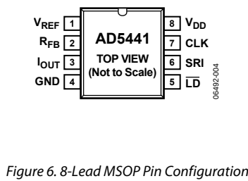
Figure 6. 8-Lead MSOP Pin Configuration
