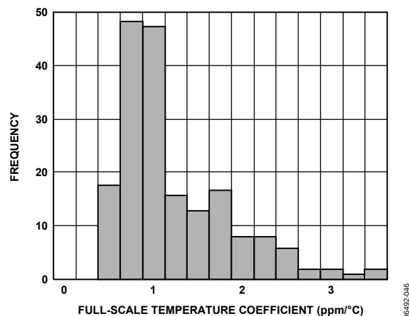
Figure 17. Full-Scale Output Temperature Coefficient Histogram
