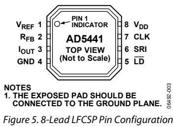
Figure 5. 8-Lead LFCSP Pin Configuration
