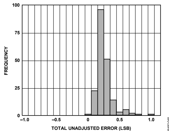
Figure 12. Total Unadjusted Error Histogram
