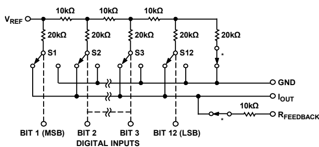
Figure 21. Simplified DAC Circuit
