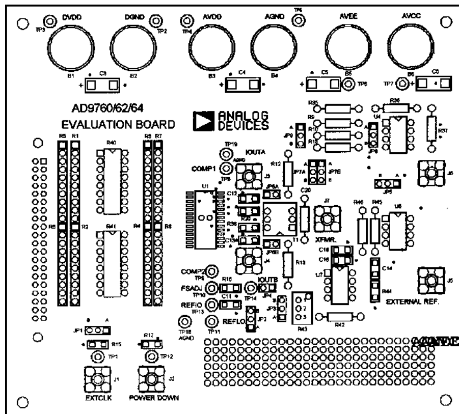
Figure 39. Silkscreen Layer—Top
