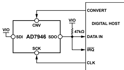
Figure 35. \overline{\text{CS}} Mode 3-Wire with BUSY Indicator Connection Diagram (SDI High)
