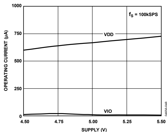
Figure 18. Operating Current vs. Supply
