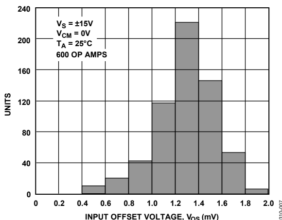
Figure 7. OP492 Input Offset Voltage Distribution @ \pm 15 V
