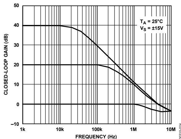
Figure 24. OP292/OP492 Closed-Loop Gain vs. Frequency @ \pm 15\text{ V}
