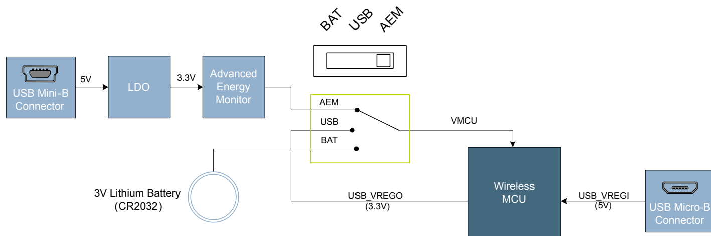
Figure 4.1. WSTK6224 Power Switch
