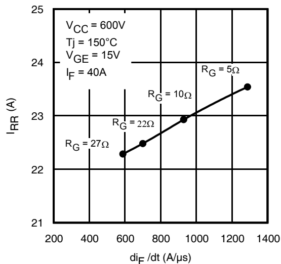
Fig. 12 - Typ. I_{RR} vs. di/dt
