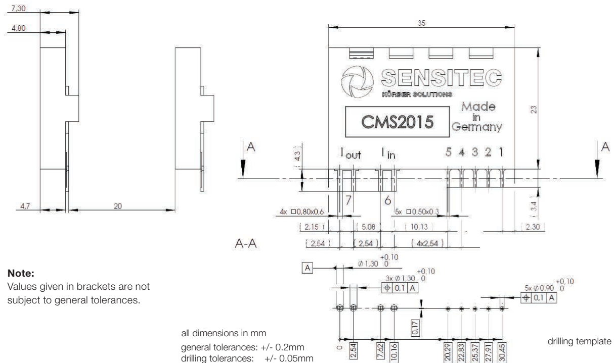
Fig. 7: Package outline.
