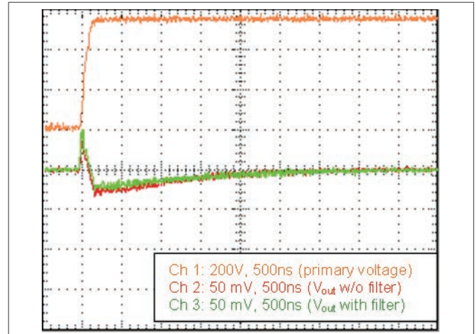
Fig. 3: dV/dt (3.7kV/ \mu\text{s} ; 530V voltage on primary conductor; filter configuration acc. to Tab. 1).
