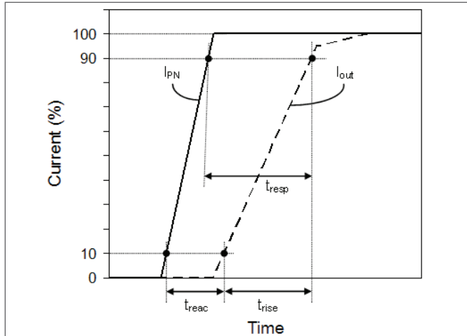
Fig. 2: Definition of reaction time ( t_{\text{reac}} ), rise time ( t_{\text{rise}} ) and response time ( t_{\text{resp}} ).
