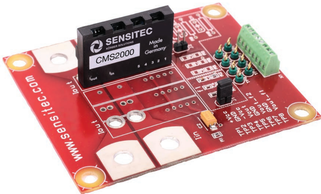
Fig. 10: The CMK2000 demoboards are available for different current ranges.
