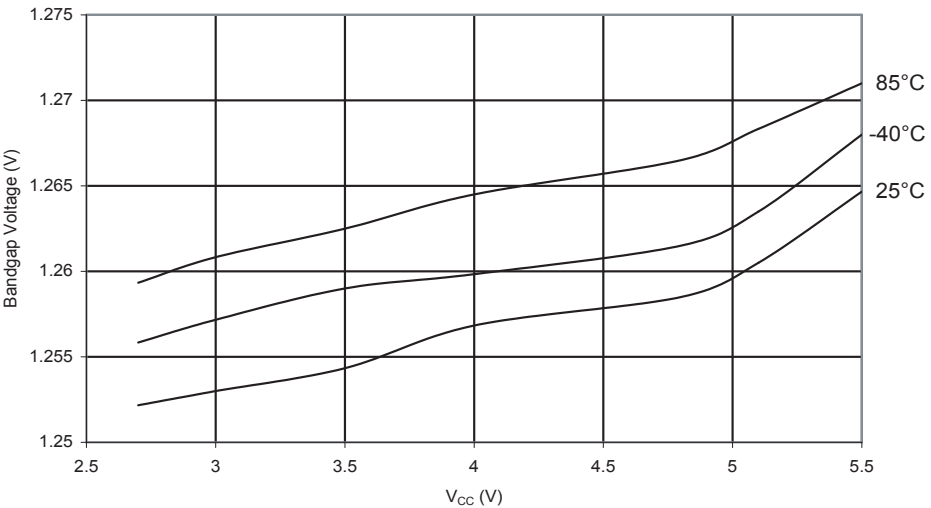
Figure 200. Bandgap Voltage vs. V_{CC}
