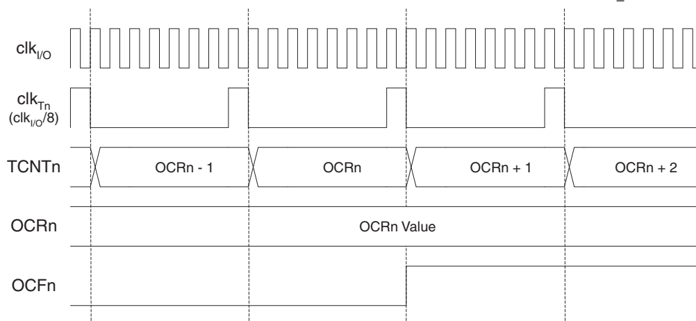
Figure 70. Timer/Counter Timing Diagram, Setting of OCF2, with Prescaler ( f_{clk\_I/O}/8 )
