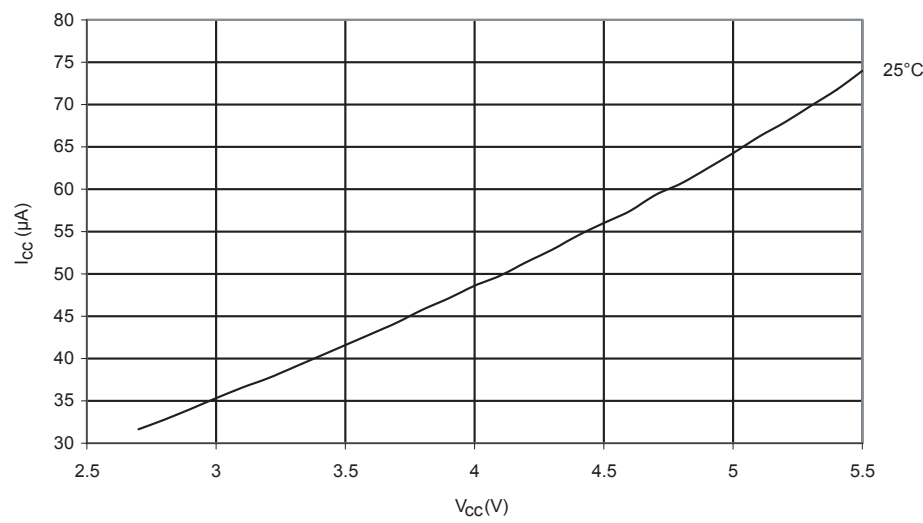
Figure 176. Idle Supply Current vs. V_{CC} (32 kHz External Oscillator)
