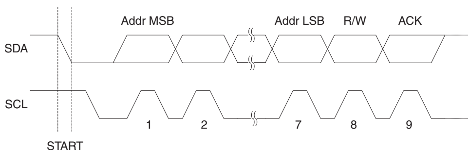
Figure 89. Address Packet Format
