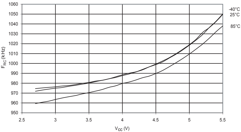
Figure 201. Watchdog Oscillator Frequency vs. V_{CC}
