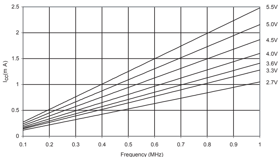
Active Supply Current Figure 163. Active Supply Current vs. Frequency (0.1 MHz - 1.0 MHz)
