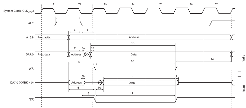
Figure 162. External Memory Timing (SRWn1 = 1, SRWn0 = 1) (1)
