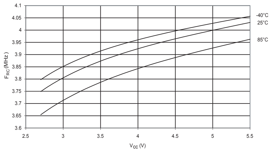
Figure 209. Calibrated 4 MHz RC Oscillator Frequency vs. V_{CC}
