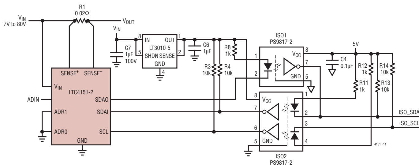
Figure 11. LTC4151-2 I²C Opto-Isolation Interface with High Speed Opto-Couplers
