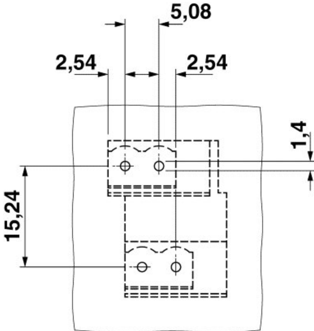
Drilling diagram
