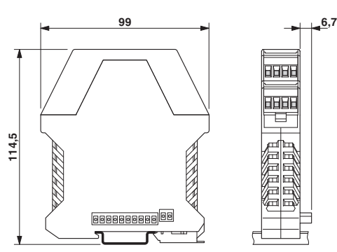
Dimensions of the electronics housing ME.../BUS 5+2 and ME.../BUS 10+2 with double-level upper part
