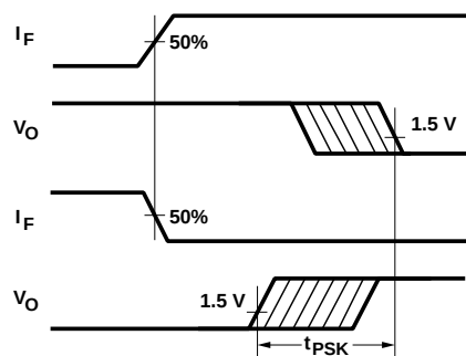
Figure 19. Illustration of Propagation Delay Skew - t_{PSK} .
