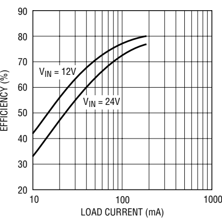
Battery Charger Efficiency— Constant V_{OUT} Region
