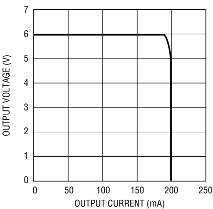
Battery Charger Output Voltage vs Output Current
