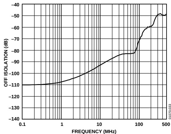
Figure 28. AD8115 Off Isolation, Input-Output
