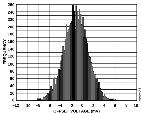
Figure 38. AD8114 Offset Voltage Distribution
