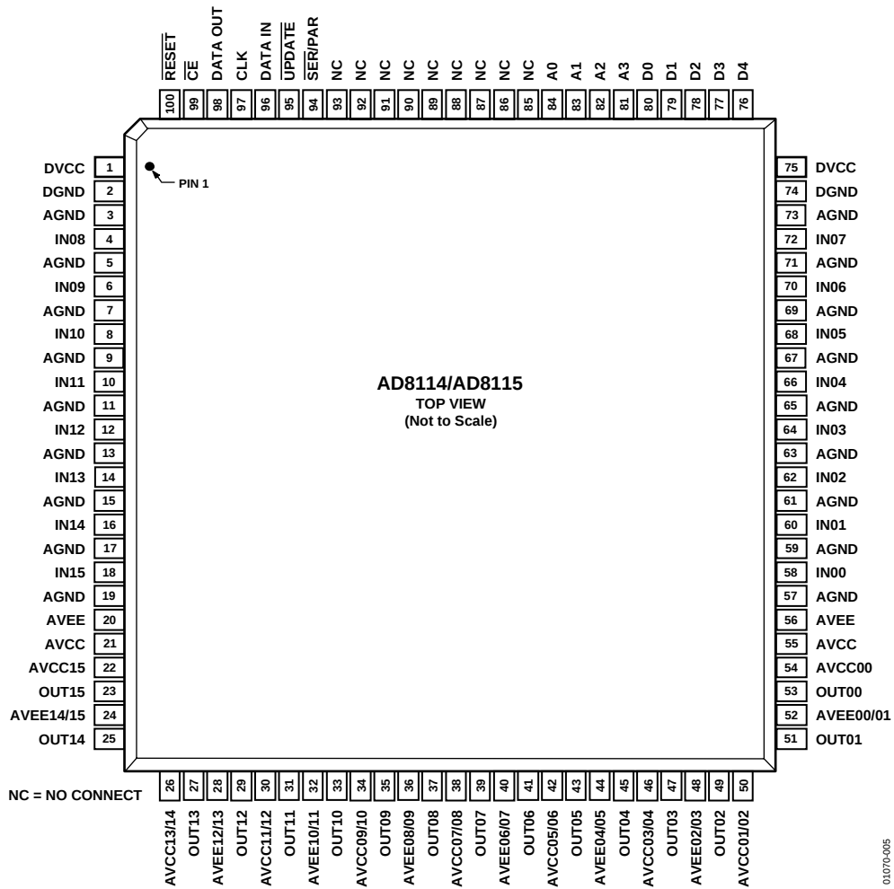
Figure 6. Pin Configuration
