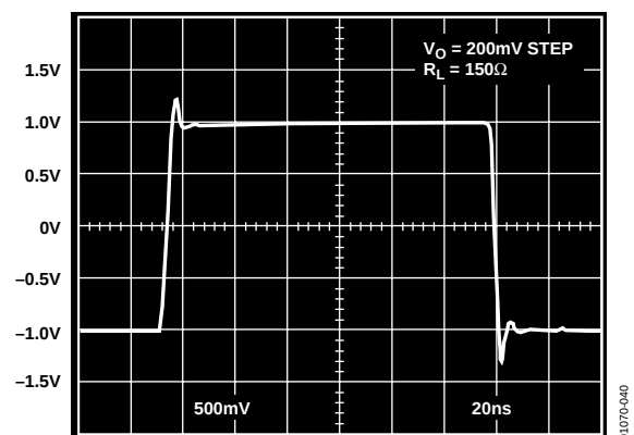
Figure 35. AD8115 Pulse Response, Large Signal
