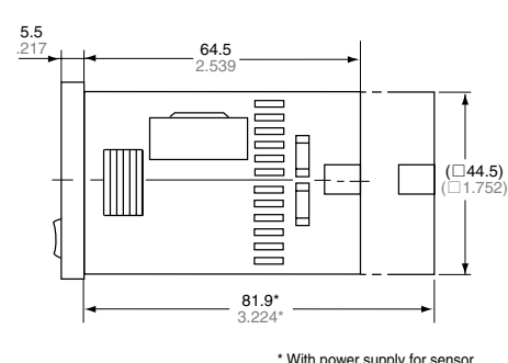
Screw terminal type: M3.5 (Flush mount)
