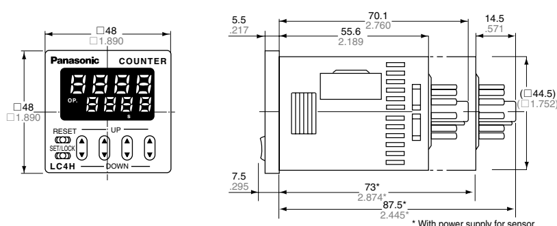
Pin type (Flush mount/Surface mount)
