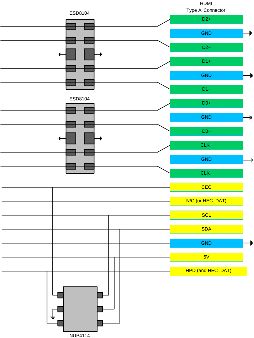
Figure 15. HDMI Layout Diagram
