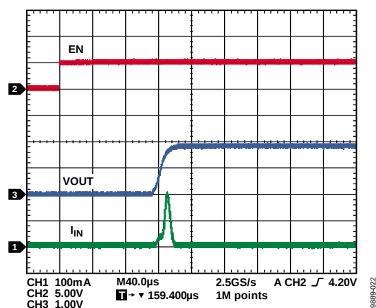
Figure 30. LDO Startup, V_{OUT3} = 1.8 \text{ V}
