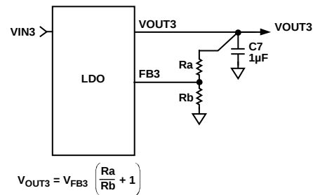
Figure 48. LDO External Output Voltage Setting
