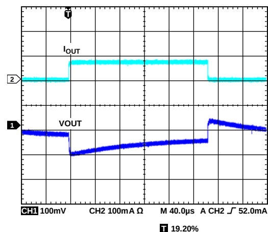
Figure 37. LDO Response to Load Transient, I_{OUT3} = 1\text{ mA} to 80\text{ mA} , V_{OUT3} = 2.8\text{ V}
