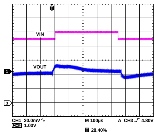
Figure 38. LDO Response to Line Transient, V_{IN} = 4.5\text{ V} to 5\text{ V} , V_{OUT3} = 2.8\text{ V}
