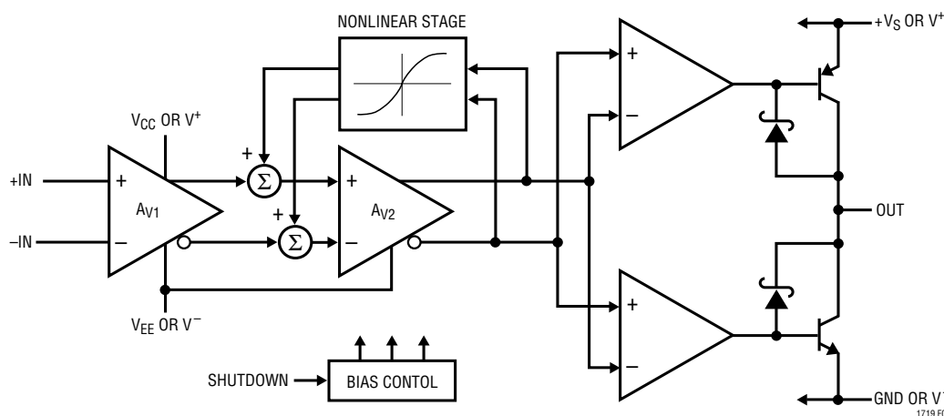
Figure 7. LT1719 Block Diagram
