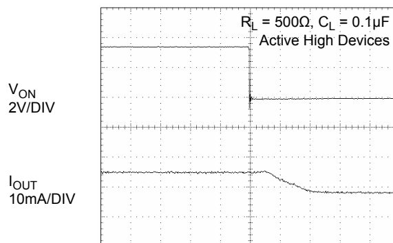
Figure 18. T OFF Response
