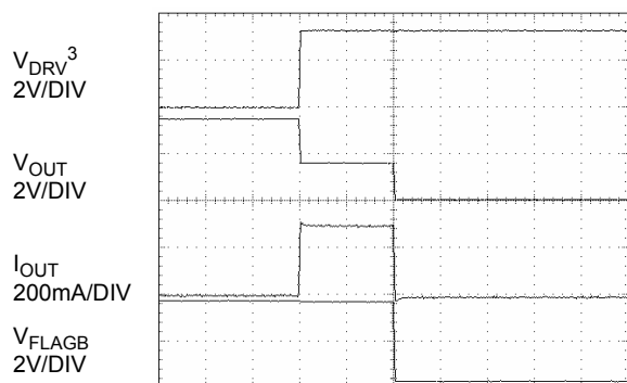
Figure 15. T BLANK Response
