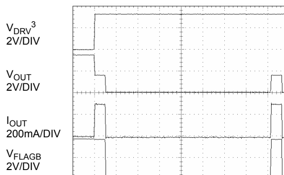
Figure 16. T RESTART Response
