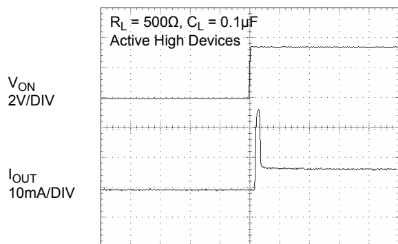
Figure 17. T ON Response
