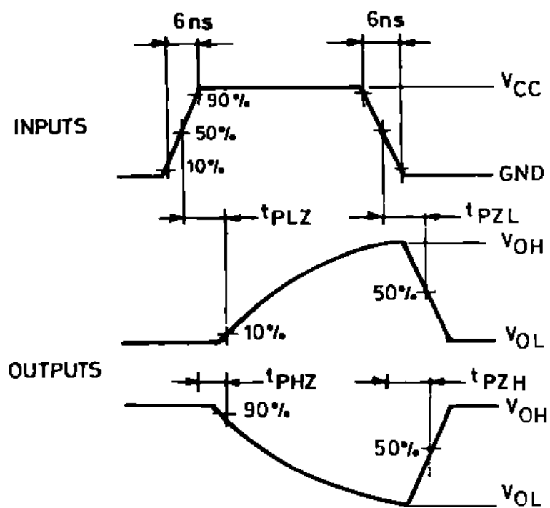
WAVEFORM 2 : OUTPUT ENABLE AND DISABLE TIME ( f=1\text{MHz} ; 50% duty cycle)
