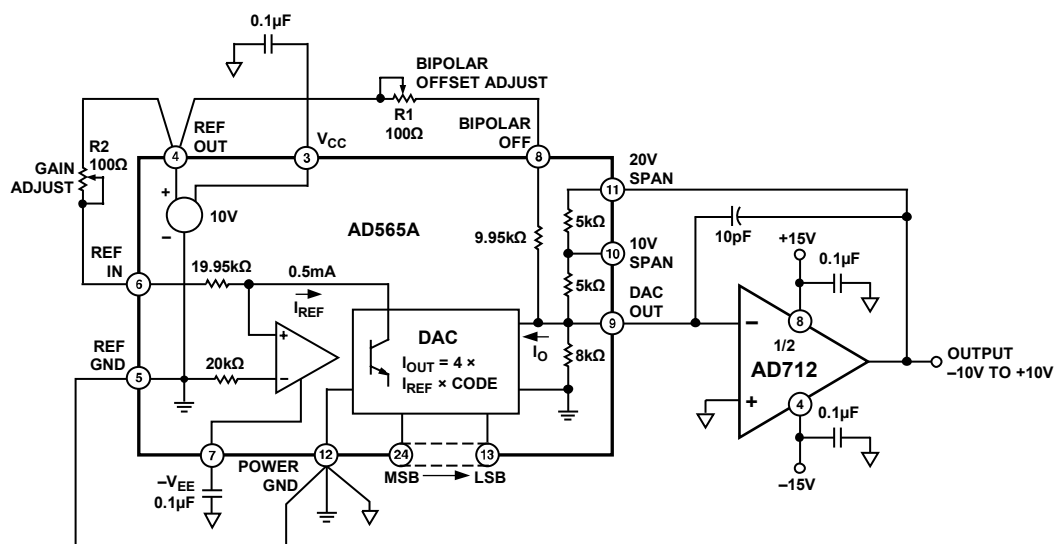
Figure 29. \pm 10 V Voltage Output Bipolar DAC
