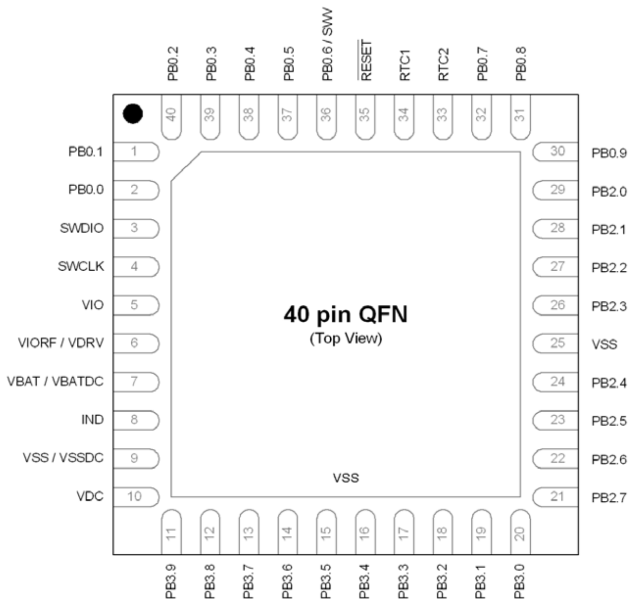
Figure 6.4. SiM3L1x4-GM Pinout
