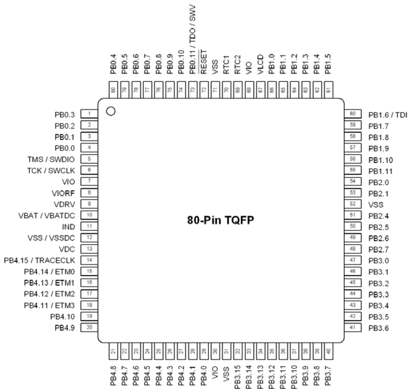
Figure 6.1. SiM3L1x7-GQ Pinout
