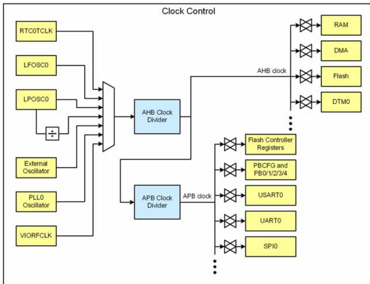
Figure 4.3. SiM3L1xx Clocking
