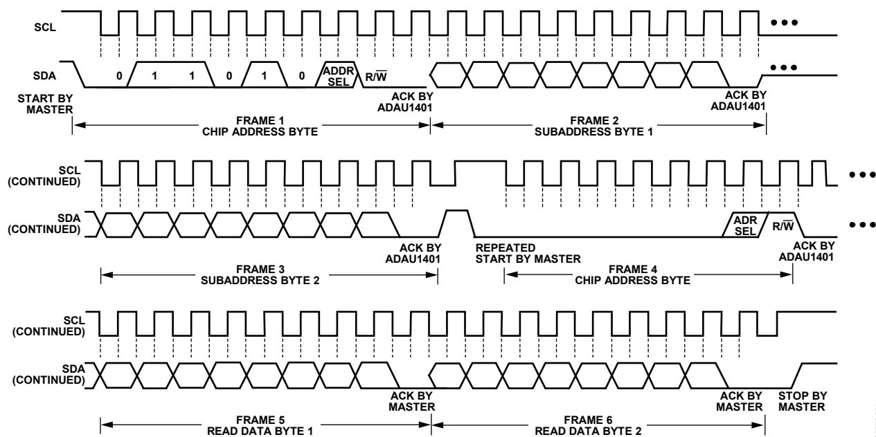
Figure 21. I²C Read from ADAU1401 Clocking
