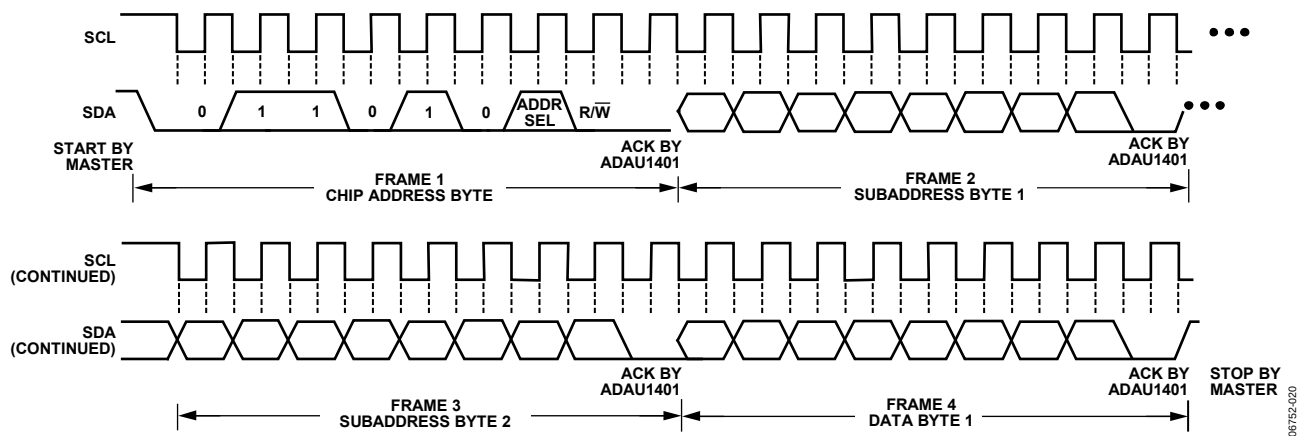
Figure 20. I²C Write to ADAU1401 Clocking
