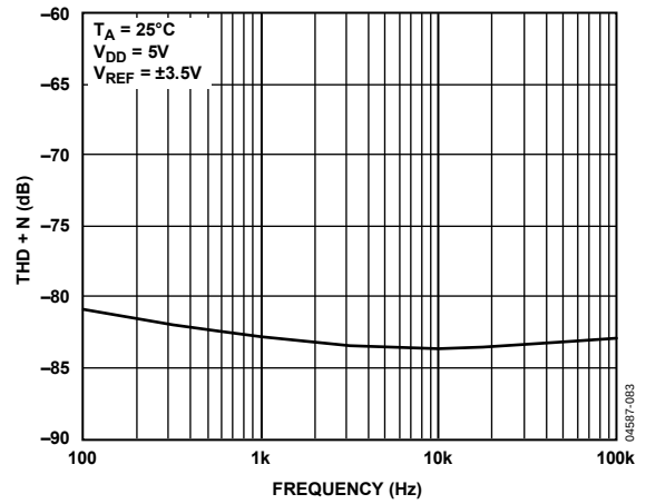
Figure 33. THD + Noise vs. Frequency
