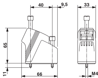
Dimensioned drawing
