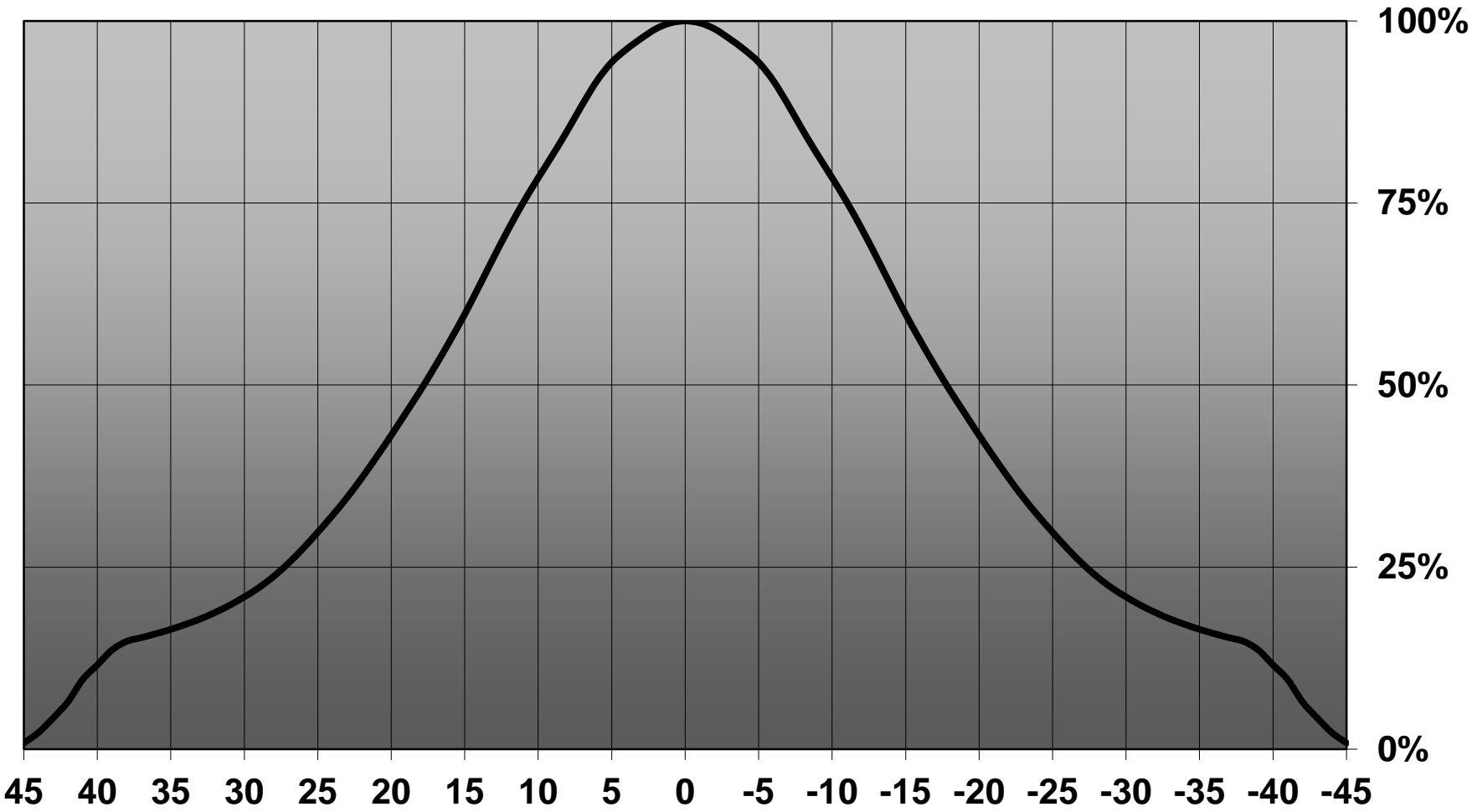
Relative intensity of C12478_MIRELLA-50-W_(OstarLighting+)
