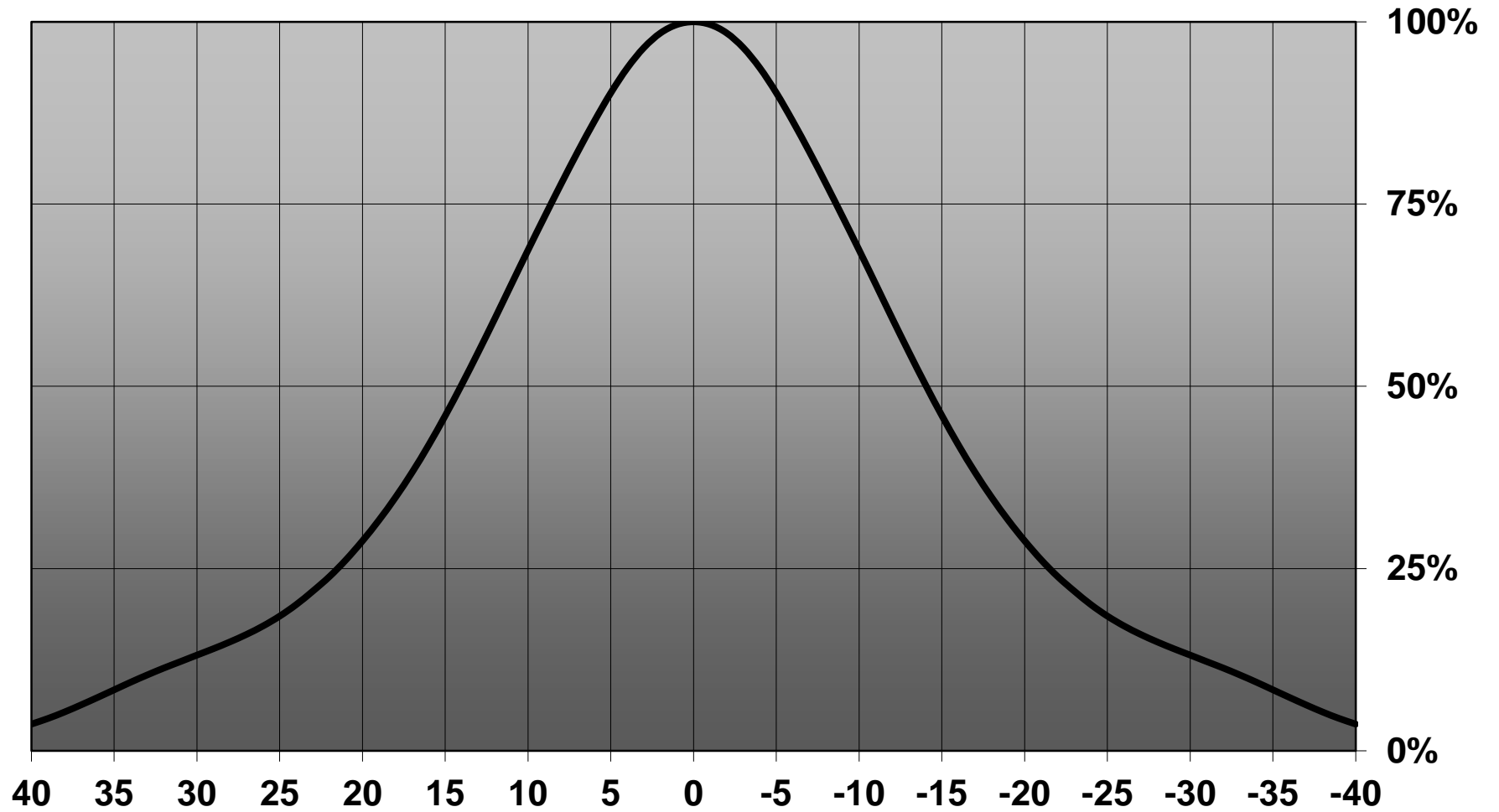
Relative intensity of CN12484_MIRELLA-50-M-DL_(OstarLighting+)
