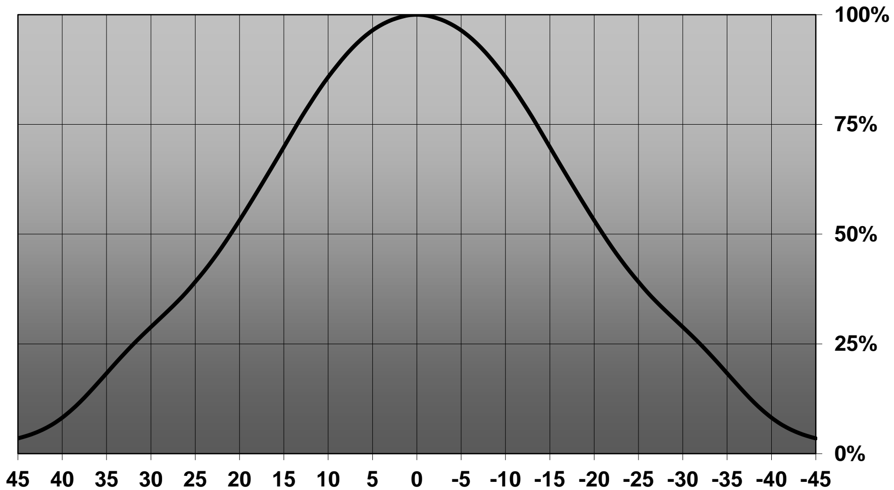
Relative intensity of CN12485_MIRELLA-50-W-DL_(OstarLighting+)
