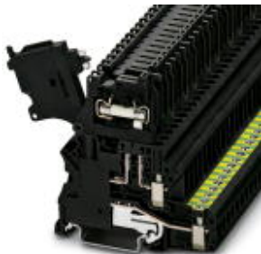
Lever-type fuse terminal block, black, for 5 x 20 mm G fuse inserts, with LED for 60 V DC
