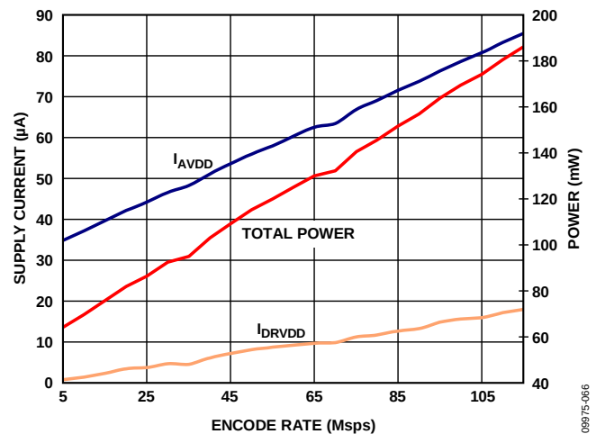
Figure 61. AD9648-105 Power and Current vs. Clock Rate (1.8 V CMOS Output Mode)
