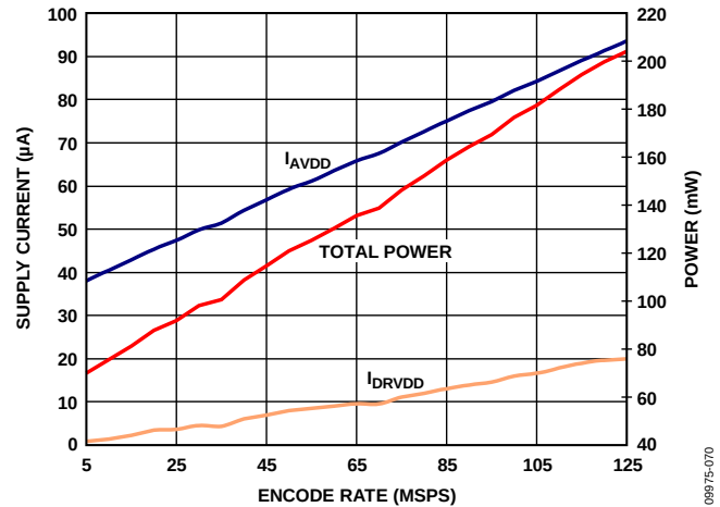
Figure 60. AD9648-125 Power and Current vs. Clock Rate (1.8 V CMOS Output Mode)
