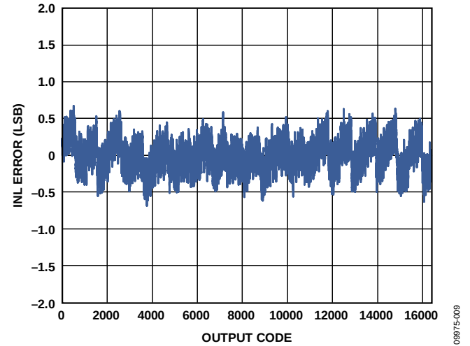
Figure 33. INL Error with f_{IN} = 9.7 MHz
