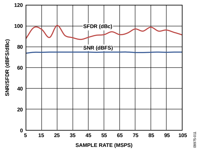
Figure 32. SNR/SFDR vs. Sample Rate with AIN = 70.1 MHz
