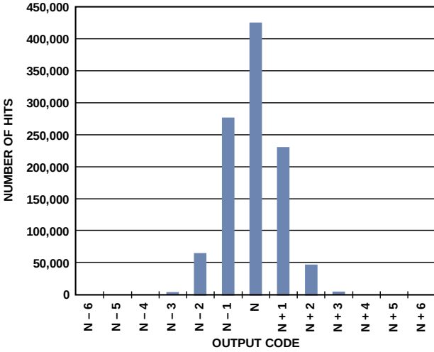
Figure 21. Shorted Input Histogram
