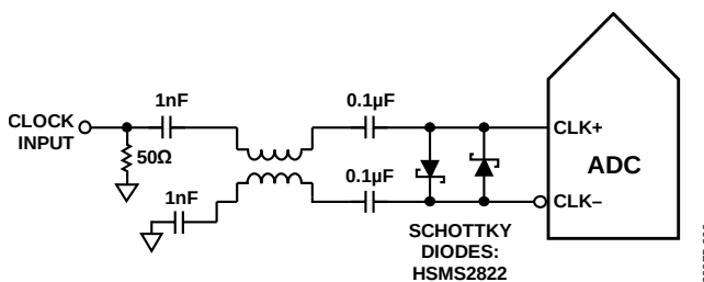
Figure 54. Balun-Coupled Differential Clock (Up to 1 GHz)
