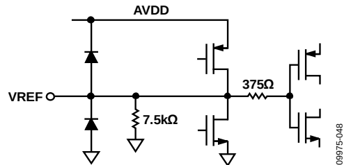
Figure 41. Equivalent VREF Circuit
