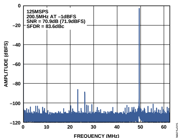
Figure 13. Single-Tone FFT with f_{IN} = 200.5 MHz
