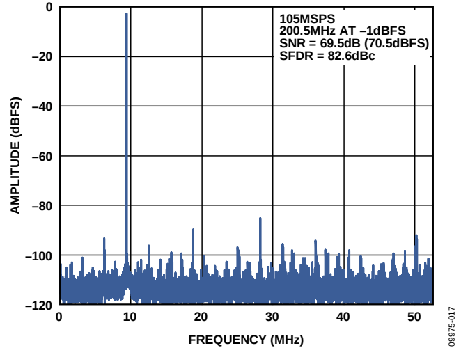
Figure 27. Single-Tone FFT with f_{IN} = 200.5 MHz
