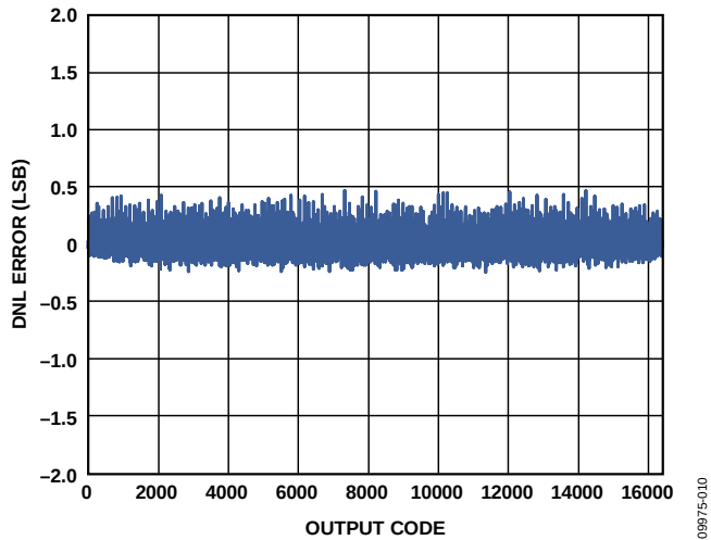
Figure 30. DNL Error with f_{IN} = 9.7 MHz
