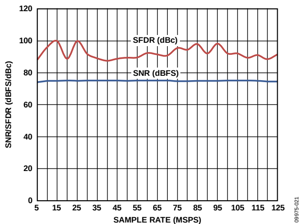
Figure 19. SNR/SFDR vs. Sample Rate with AIN = 70.1 MHz
