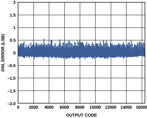
Figure 20. DNL Error with f_{IN} = 9.7 MHz
