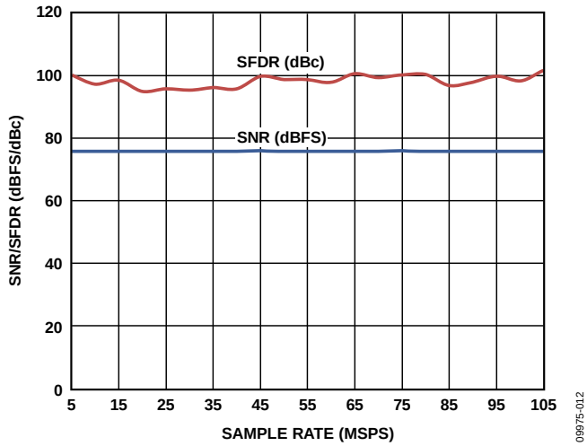
Figure 29. SNR/SFDR vs. Sample Rate with AIN = 9.7 MHz
