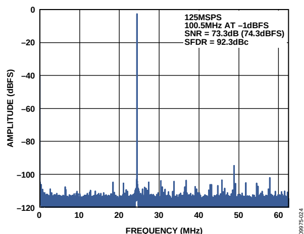
Figure 12. Single-Tone FFT with f_{IN} = 100.5 MHz
