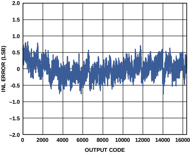
Figure 22. INL Error with f_{IN} = 9.7 MHz
