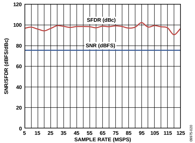
Figure 18. SNR/SFDR vs. Sample Rate with AIN = 9.7 MHz
