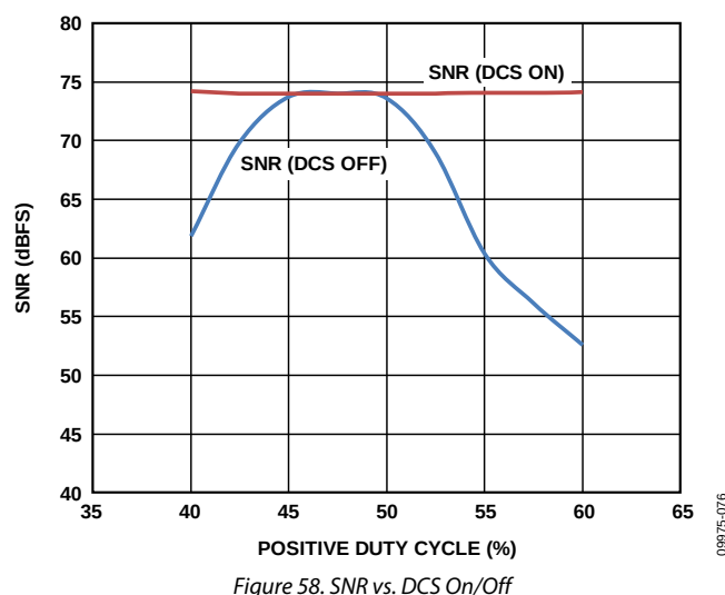
Figure 58. SNR vs. DCS On/Off
