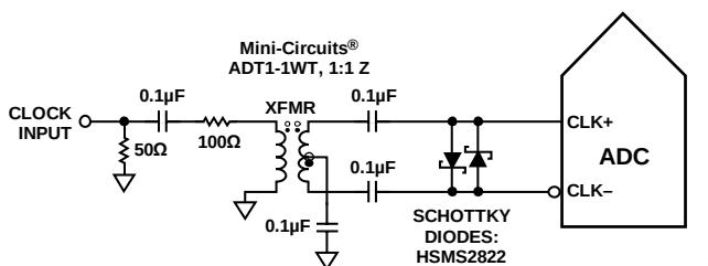
Figure 53. Transformer-Coupled Differential Clock (Up to 200 MHz)
