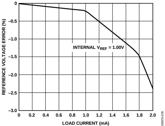
Figure 50. V_{REF} Accuracy vs. Load Current
