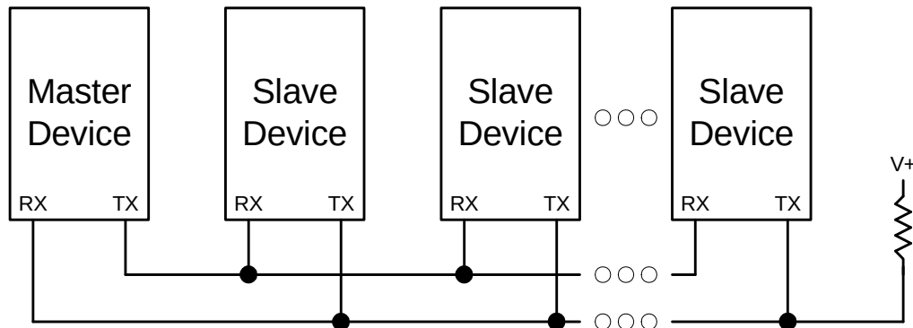
Figure 26.6. UART Multi-Processor Mode Interconnect Diagram
