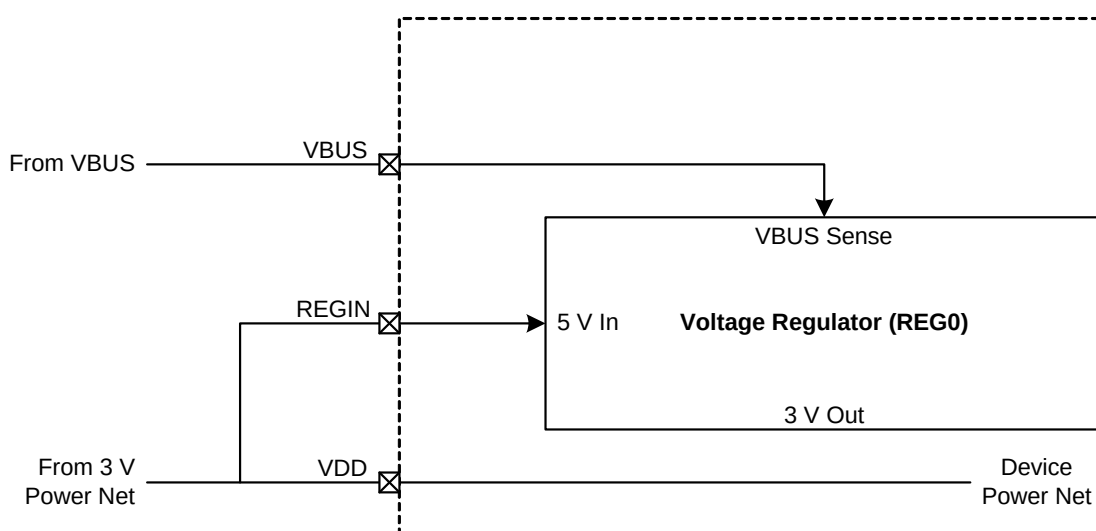
Figure 11.3. REG0 Configuration: USB Self-Powered, Regulator Disabled
