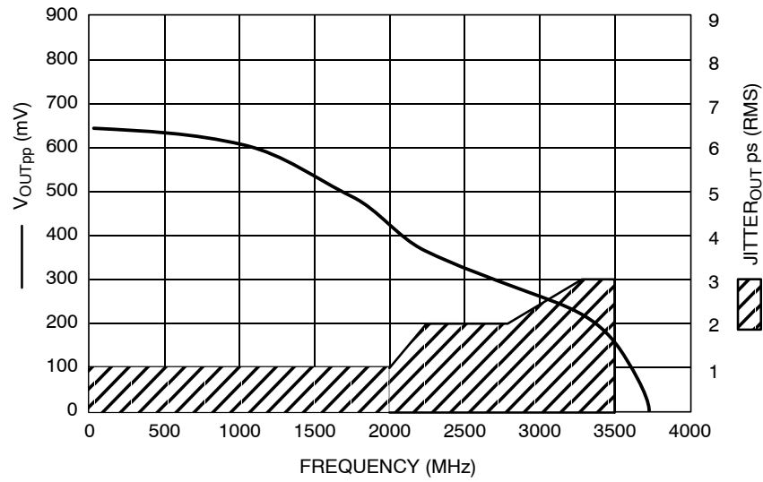
Figure 3. F_{max} /Jitter for \overline{Q} Output
