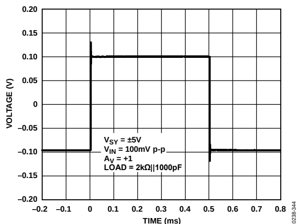
Figure 47. Small Signal Transient Response, V_{SV} = \pm 5V
