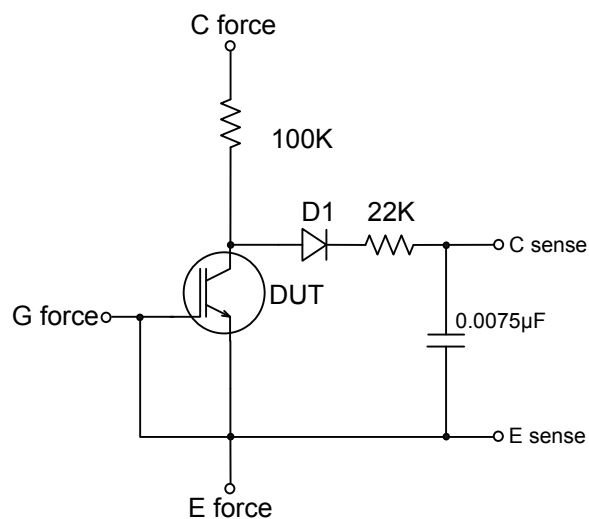
Fig.C.T.4 - Switching Loss Circuit
