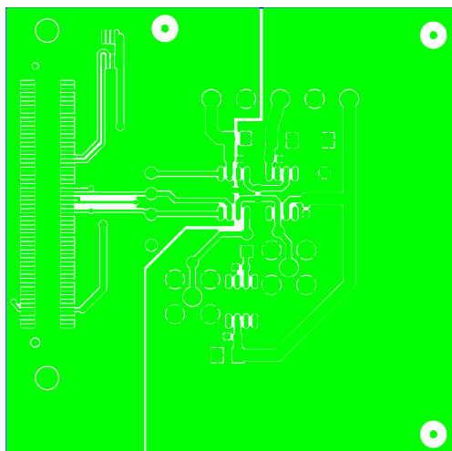
Figure 30 Component Side Artwork
