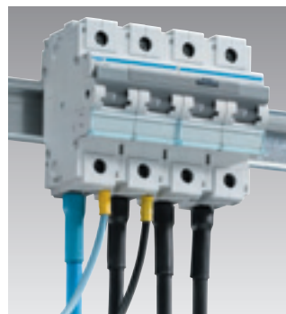
The connection of auxiliaries becomes easy, thanks to the new "Fast on" connection terminals provided on the top and bottom of the MCBs. This provides a quick and easy solution to feed auxiliaries such as shunt trip coil, UV release etc.
