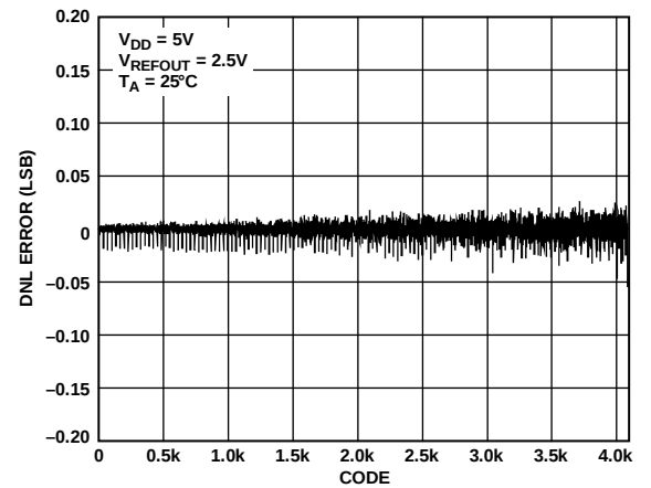
Figure 15. DNL—AD5623R-5
