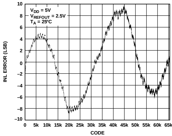
Figure 10. INL—AD5663R-5
