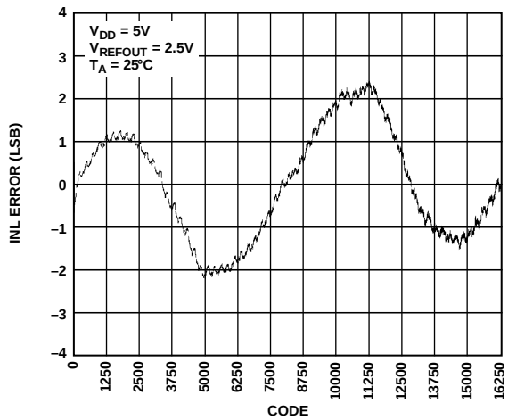
Figure 11. INL—AD5643R-5
