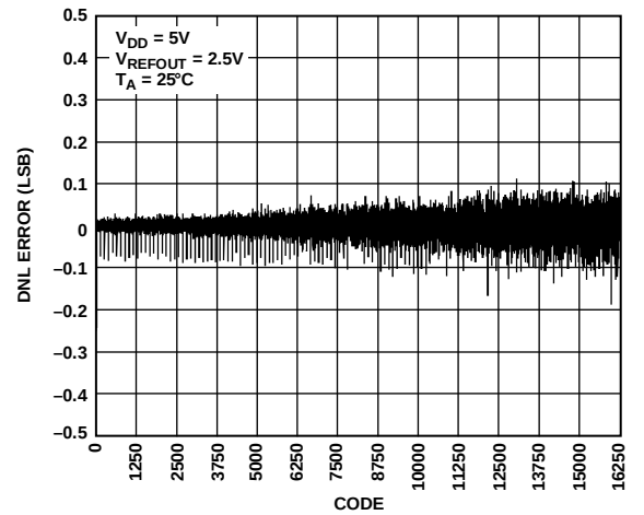
Figure 14. DNL—AD5643R-5
