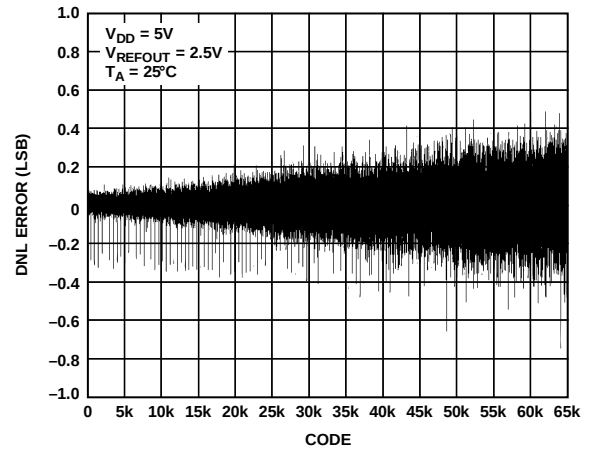
Figure 13. DNL—AD5663R-5
