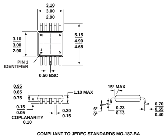
Figure 64. 10-Lead Mini Small Outline Package [MSOP] (RM-10) Dimensions shown in millimeters
