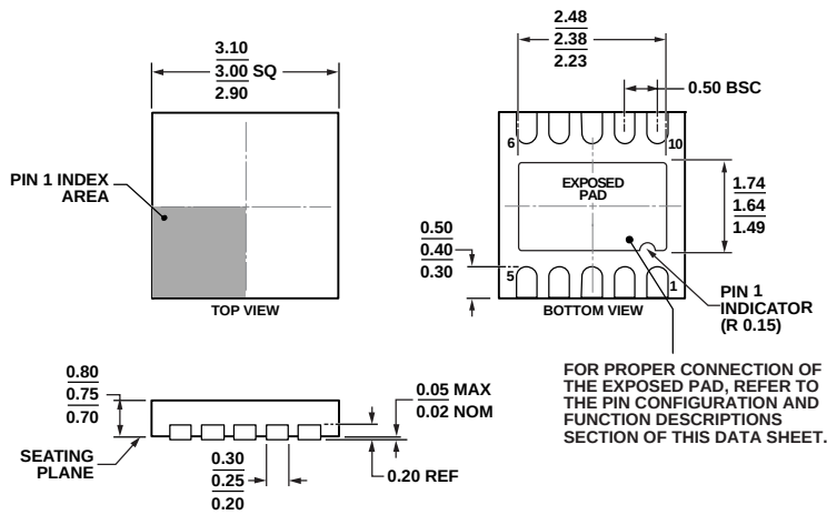
Figure 63. 10-Lead Lead Frame Chip Scale Package [LFCSP_WD] 3 mm x 3 mm Body, Very Very Thin, Dual Lead (CP-10-9) Dimensions shown in millimeters
