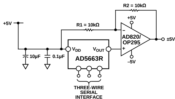
Figure 61. Bipolar Operation with the AD5663R
