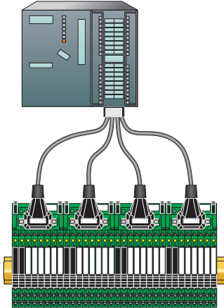
Wiring with V8 adapter
