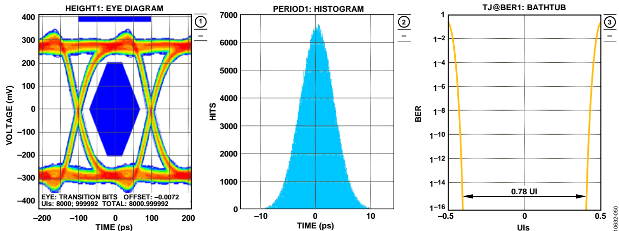
Figure 54. AD6673 Digital Outputs Data Eye, Histogram, and Bathtub, External 100 Ω Terminations at 5 Gbps
