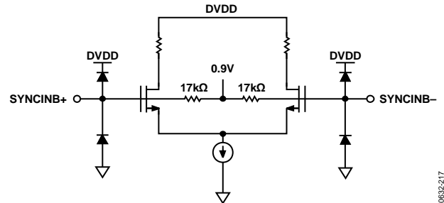
Figure 22. Equivalent SYNCINB± Input Circuit
