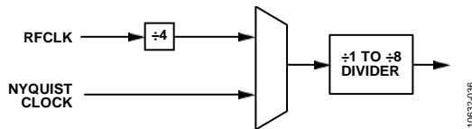
Figure 40. AD6673 Clock Divider Circuit
