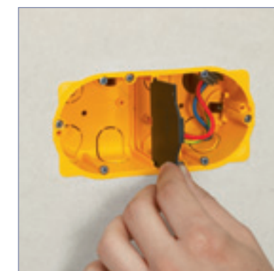
Large volume de câblage Cloison amovible
