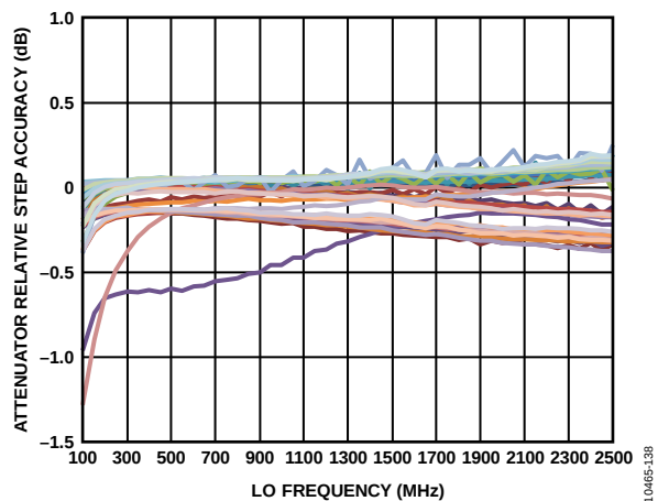
Figure 37. Attenuator Relative Step Accuracy over all Attenuation Steps vs. LO Frequency, Nominal Conditions
