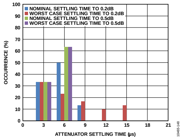
Figure 49. Attenuator Settling Time to 0.2 dB and 0.5 dB Distribution at Nominal and Worst-Case Conditions for Typical Large Step
