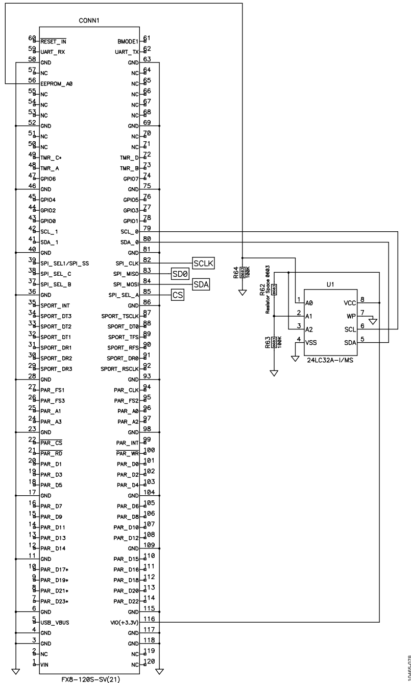
Figure 71. Applications Circuit Schematic—SDP-S
