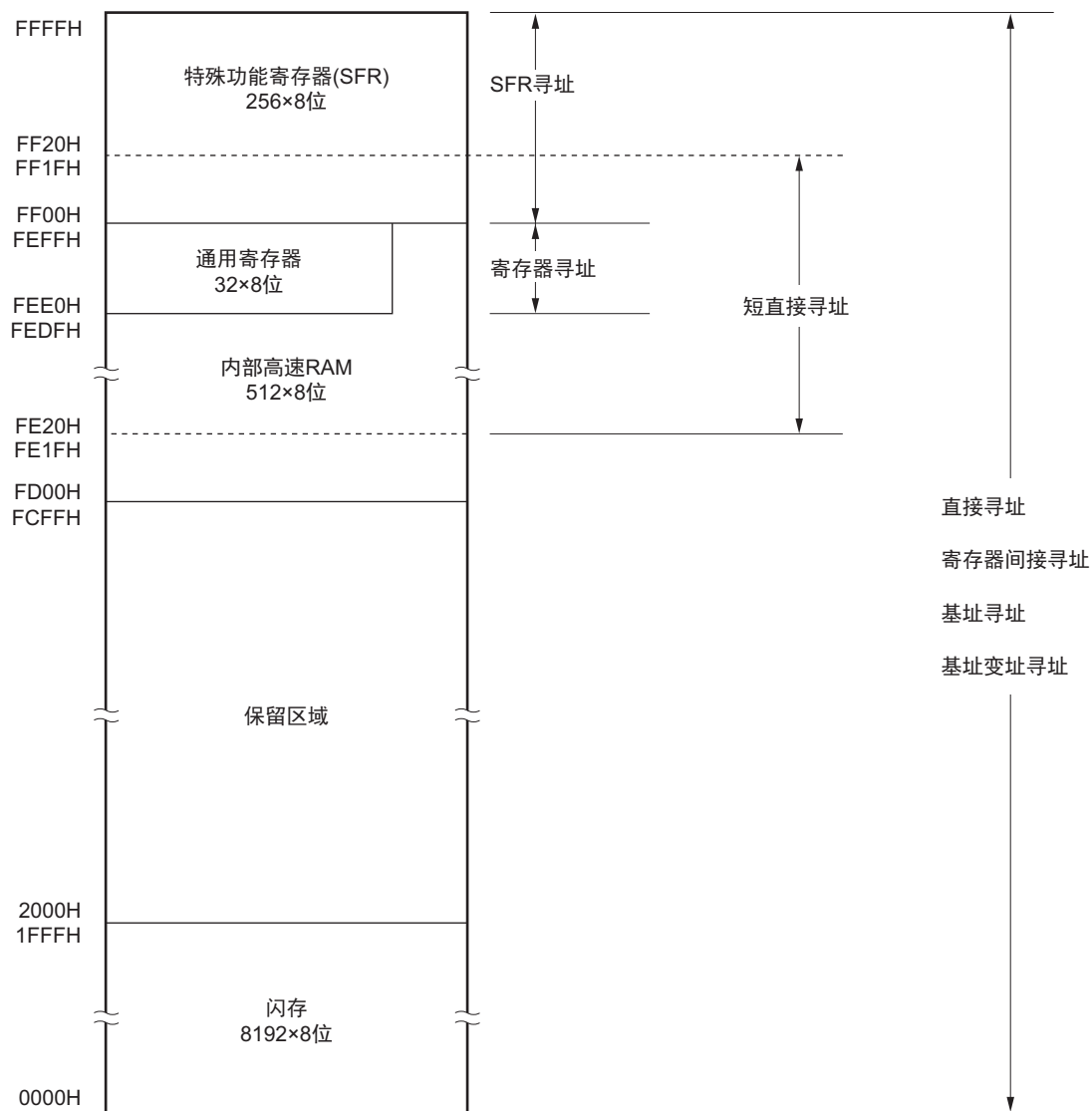
图 3-5 数据存储与寻址的对应 (R7F0C301x、R7F0C304x、R7F0C307x、R7F0C310x)
