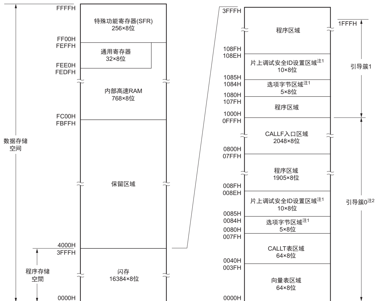
图 3-3 存储器映射图 (R7F0C302x、R7F0C305x、R7F0C308x、R7F0C311x)
