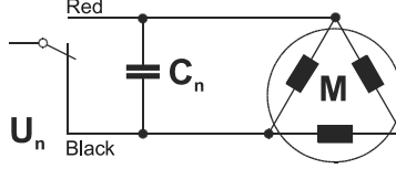
UFR3 Parallel circuit
